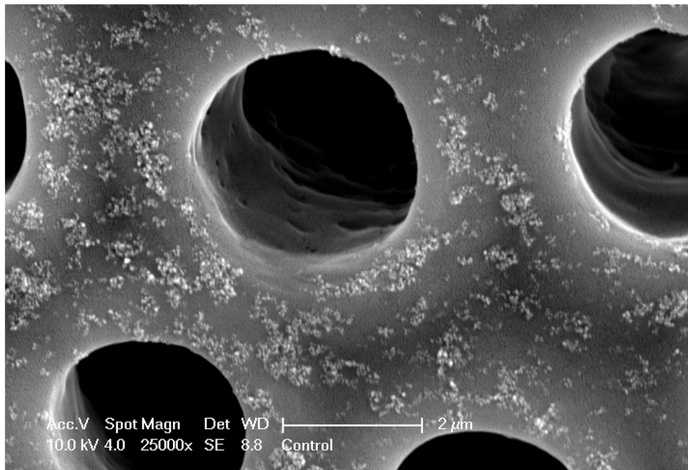
Fig. 4. Scanning electron microscopy image of a mid-coronal crown dentin that was acid-etched for 15 sec with 37% phosphoric acid, rinsed with water for 10 sec and then air-dried for 30 sec with continuous air blast at a distance of 10 cm (25,000x). Fine granular materials present on the surface of the collapsed intertubular dentin is silica gel used by 3M to gel their phosphoric acid etchant. No individual collagen fibrils could be identified on the surface of the intertubular dentin or within the walls of the dentinal tubules because they have fused with each other by direct hydrogen bonding [7].
